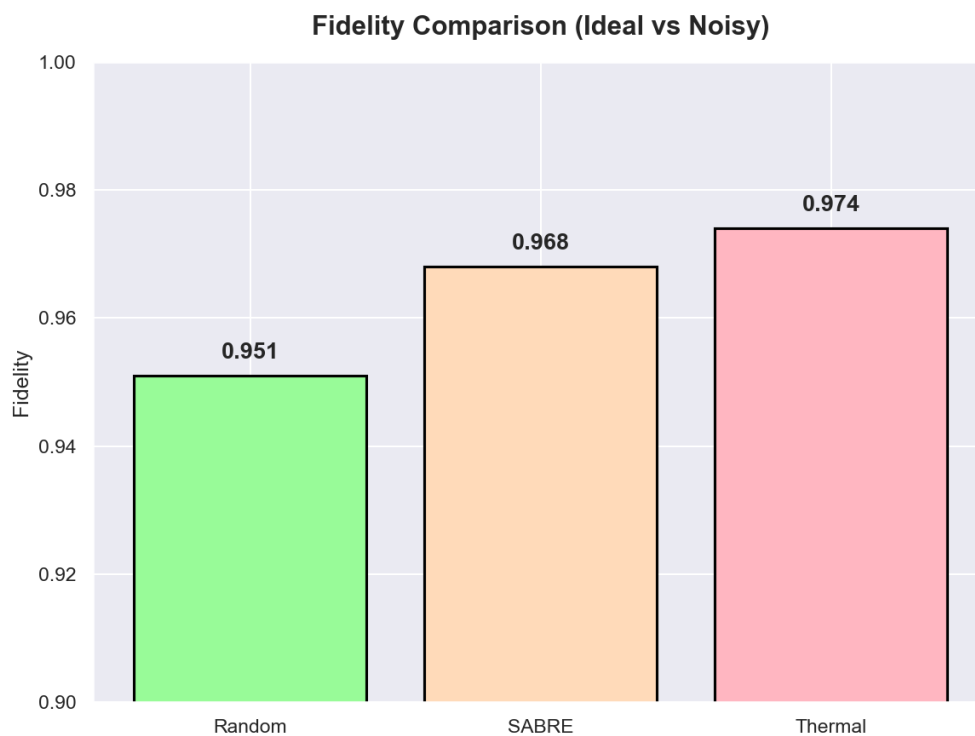
Fig. 4. Fidelity Comparison (Ideal vs. Noisy) across Random, SABRE, and Thermal-Aware mapping strategies.
