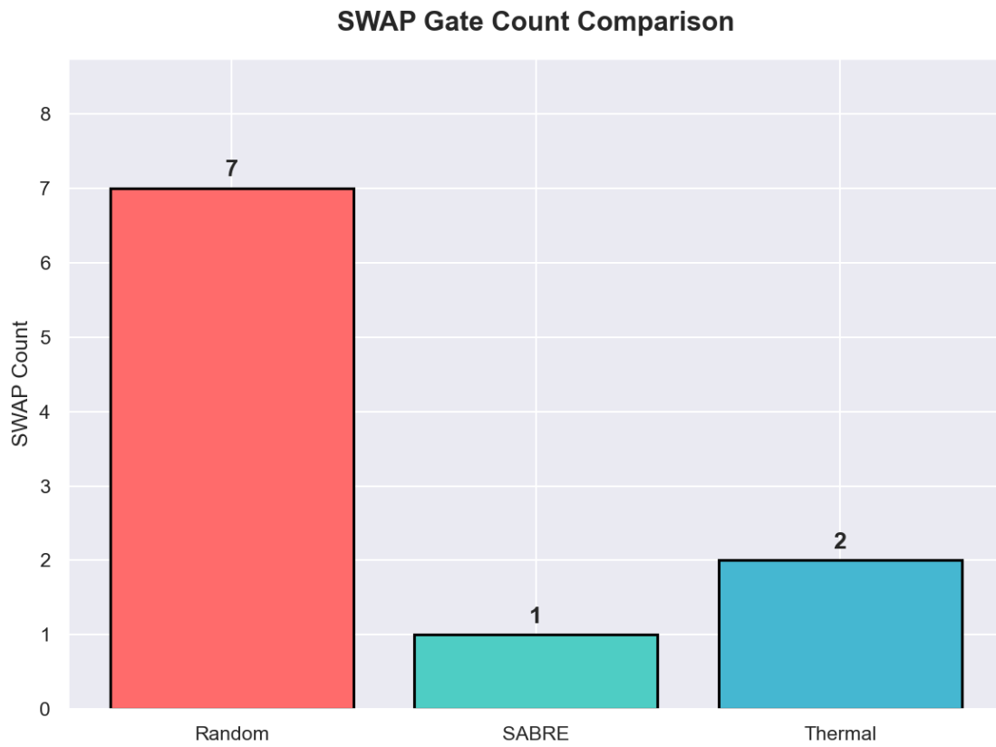
Fig. 2. SWAP Gate Count Comparison across Random, SABRE, and Thermal-Aware mapping strategies.
