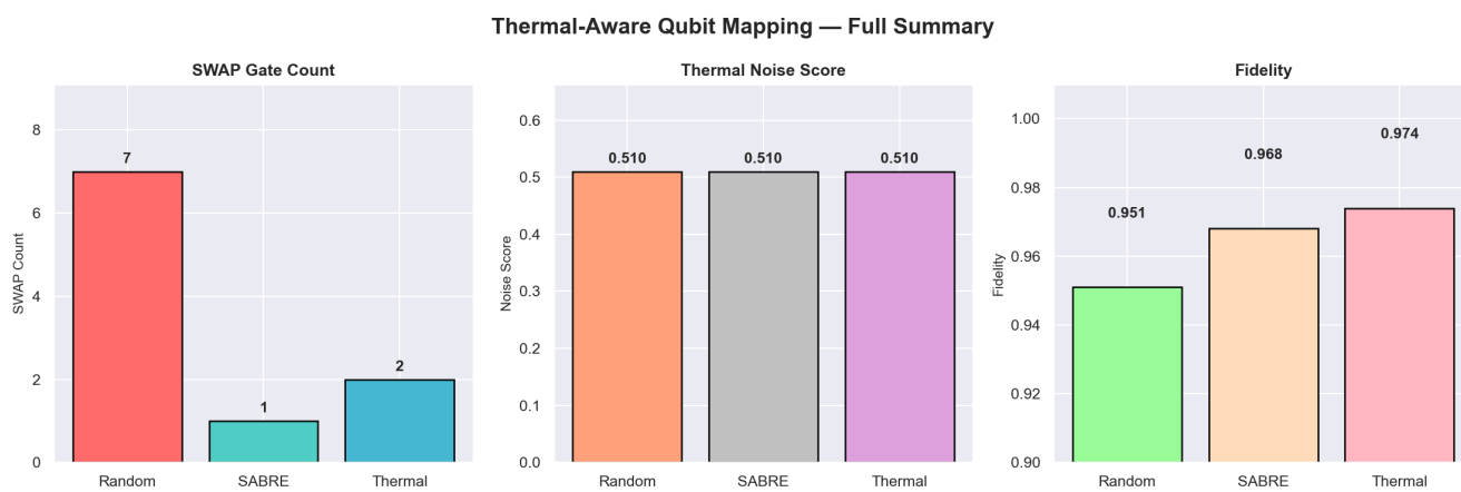
Fig. 5. Full summary of thermal-aware qubit mapping results: SWAP gate count, thermal noise score, and fidelity.
